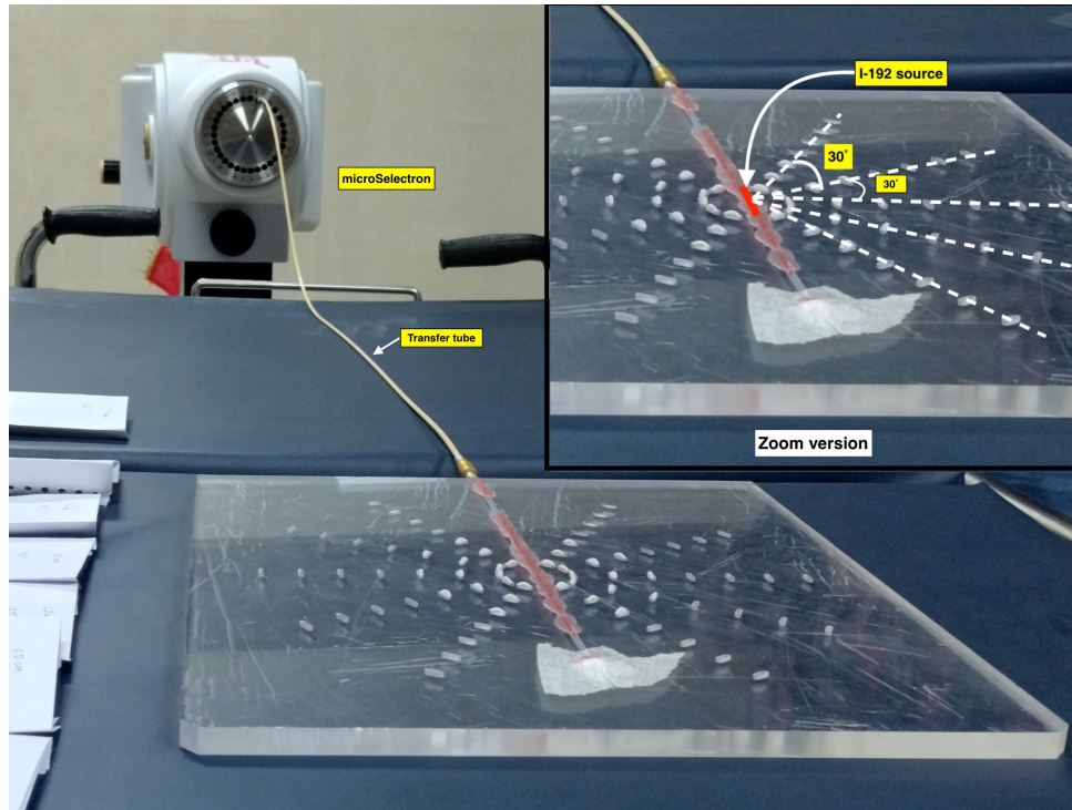
Figure 2: Experimental setup used for in-phantom dosimetry measurements.
