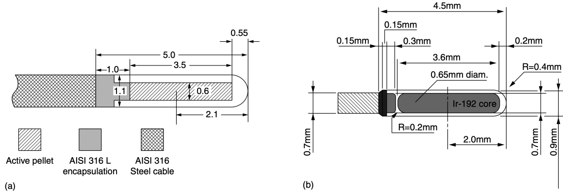
Figure 3: MicroSelectron HDR 192Ir source type designs (Nucletron B.V ., Veenendaal, The Netherlands). (a) The old “classic” design with 0.6 mm cylindrical core diameter and 3.5 mm core length having a total outer diameter (including encapsulation) of 1.1 mm.20 (b) The new design with a cylindrical core diameter of 0.65 mm and core length of 3.6 mm. The total outer diameter of this source design is 0.9 mm (figure provided by Nucletron). All dimensions shown are in mm.
