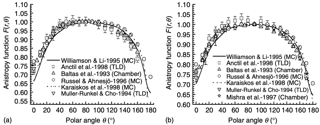
Figure 5: Comparison of the anisotropy function, F(r, u) , values published by several authors, estimated either experimentally or using MC simulations for the microSelectron HDR 192Ir type old “classic” source at radial distance (a) r = 3.0 cm and (b) r = 5.0 cm.
