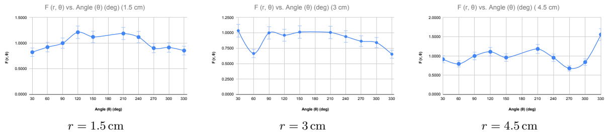
Figure 4: Anisotropy function F(r, \theta) at different radial distances
